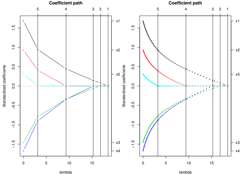
Figure 1: In the left panel, the exact solutions were computed at the values of \lambda where the active set changed, and the solutions were connected in a piecewise linear manner. The right panel shows the paths with exact solutions at much finer grids of \lambda ; we controlled the arc length to be less than 0.1 between any two adjacent values of \lambda .
