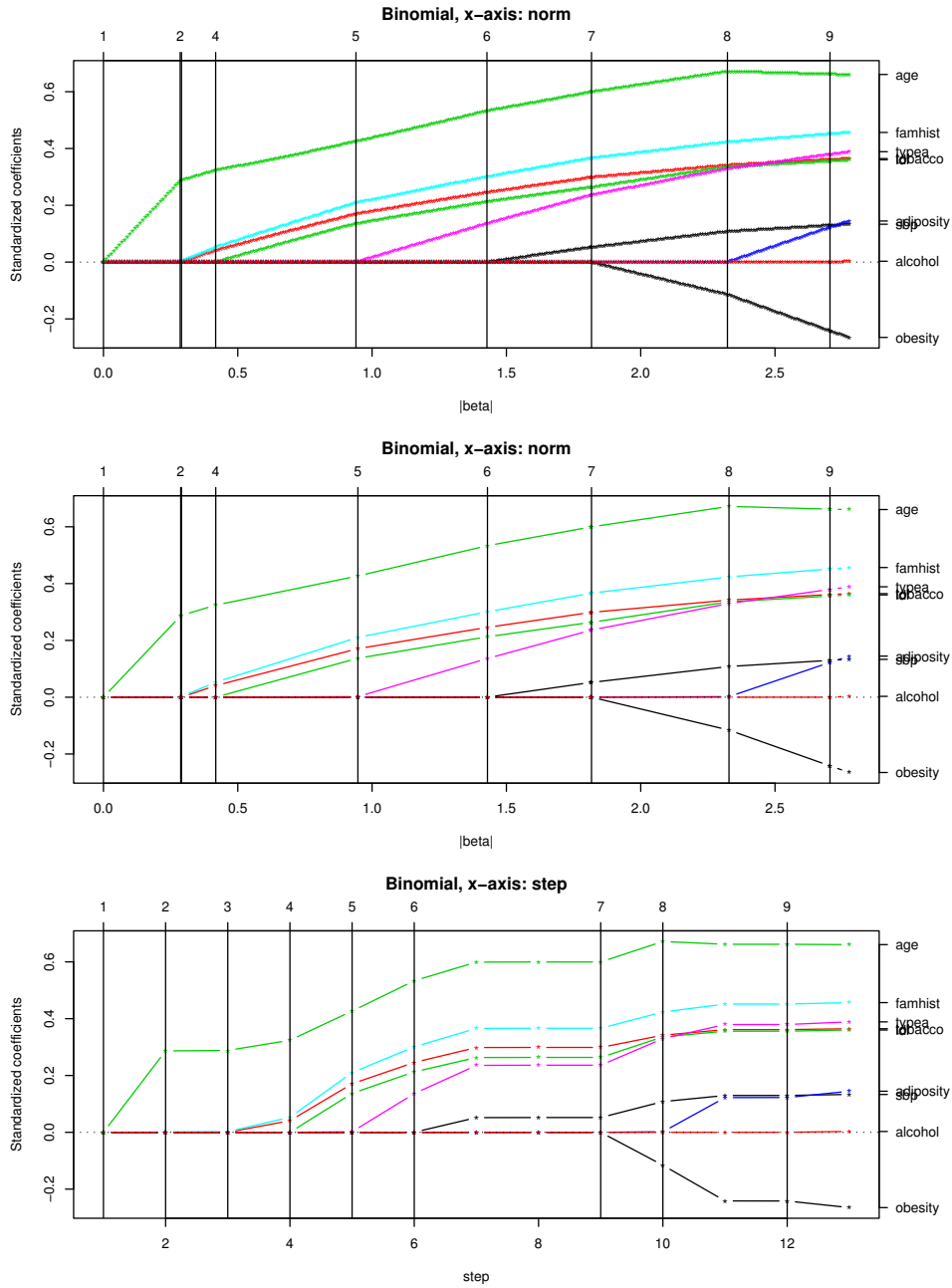
Figure 2: The first plot shows the exact set of paths; the coefficients were precisely computed at 300 different grids of \lambda ranging from 81.9 to 0, with the constraint that every arc length be less than 0.01. The vertical breaks indicate where the active set is modified, and the L_1 norm of the coefficients forms the x-axis. Comparing this plot to the second panel, which we achieved in 13 steps rather than 300, we find that the two are almost identical. The bottom panel represents the paths as a function of step-number, to illustrate how minor the corrections are.
