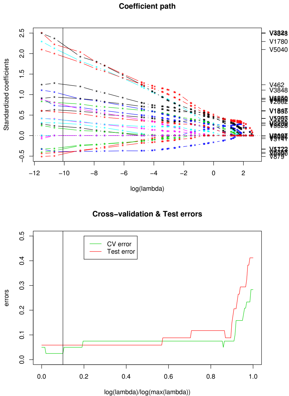
Figure 4: The first panel shows the coefficient paths we achieved using the training data; the size of the active set cannot exceed the sample size at any segment of the paths. The vertical line marks the chosen level of regularization (based on cross-validation), where 23 variables had nonzero coefficients. The second panel illustrates the patterns of 10-fold cross-validation and test errors. As indicated by the vertical line, we selected \lambda where the cross-validation error achieved the minimum.
